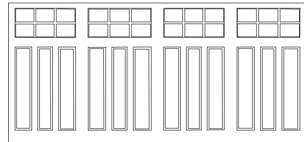
14'0" x 7'0" Option2 (4276 x 2134)
