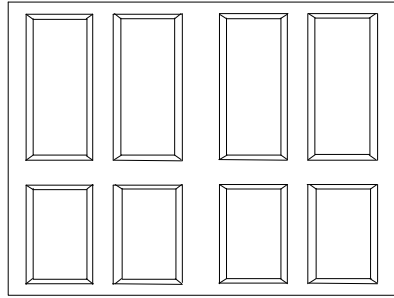
9'0" x 7'0" (2743 x 2134)
